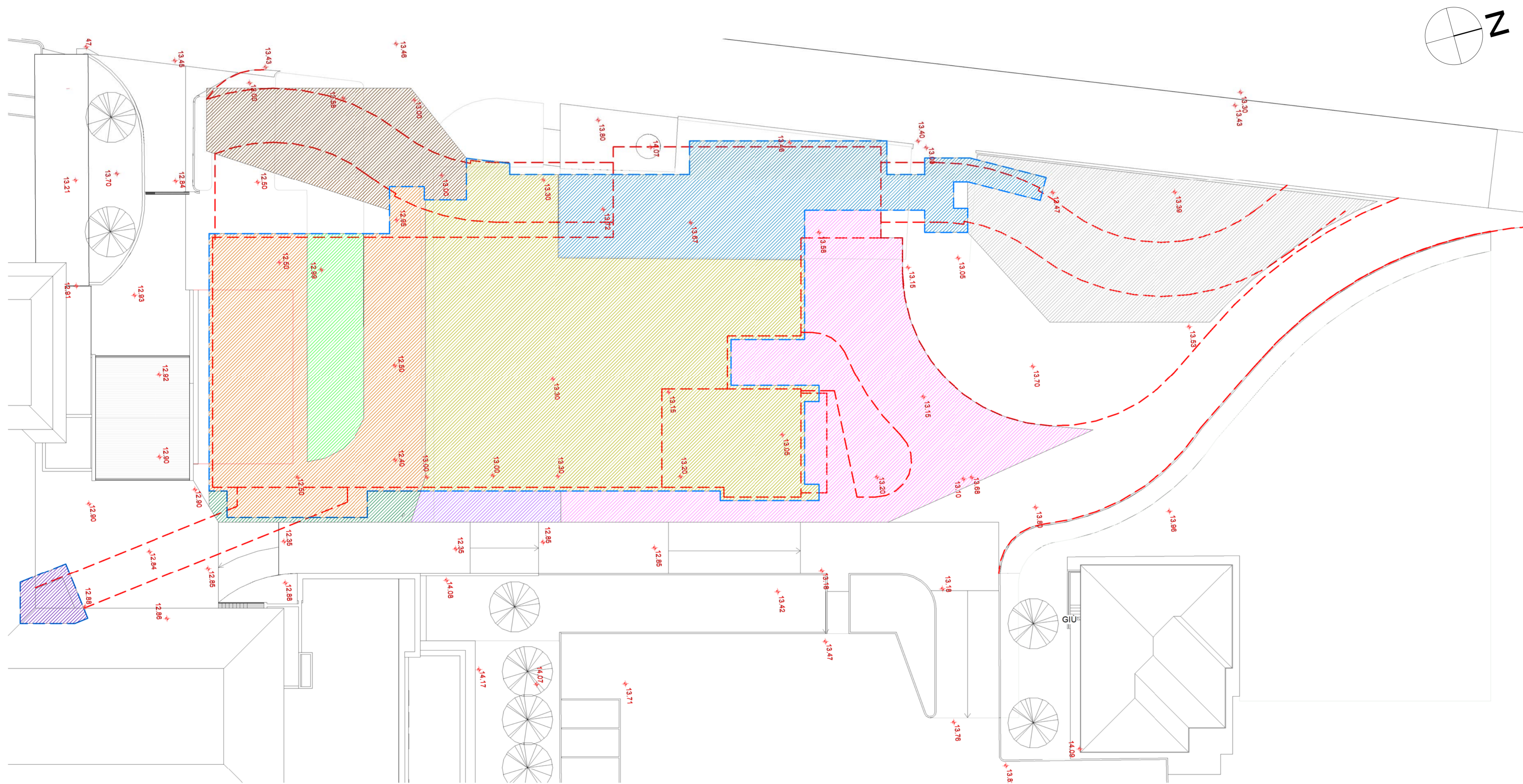
Planimetria Interventi-Scavi 1 : 200
